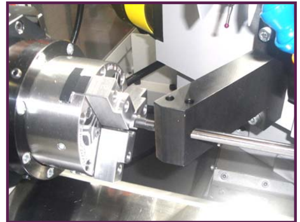
Boring bar attachment to machine chuck jaws
