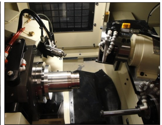
Angular OD wheel for precision shoulder & face grinding
