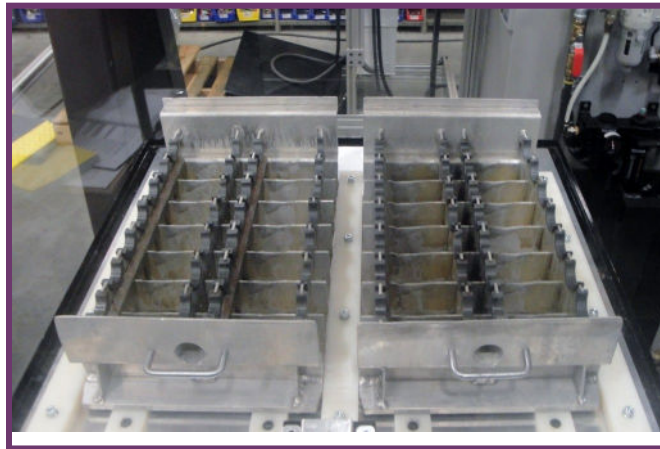
Dual tray station, holds 14 parts per tray
