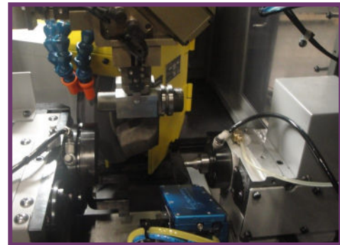
Tailstock with custom center
