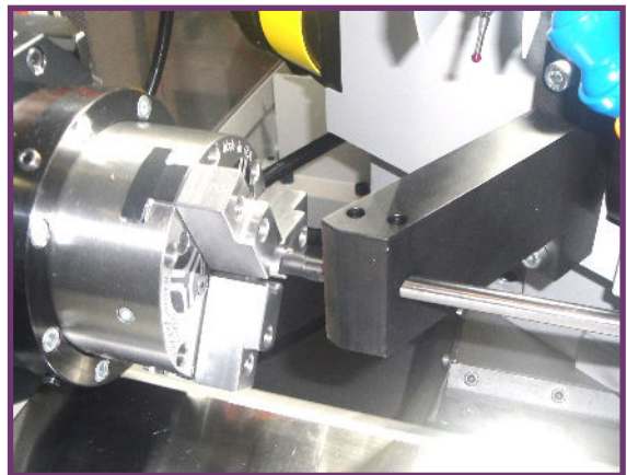
Boring bar attachment to machine chuck jaws
