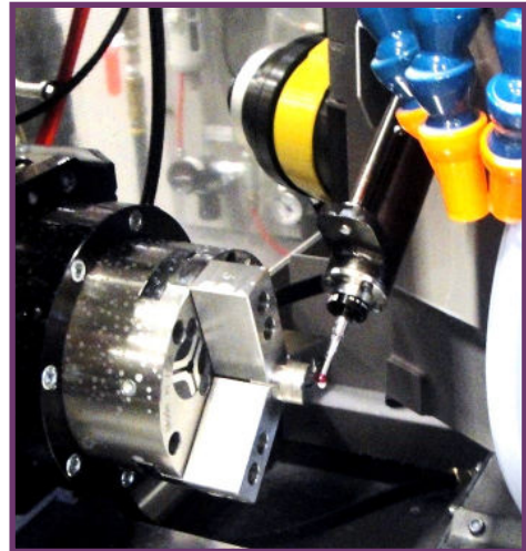
Automatic lateral locator with Renishaw probe
