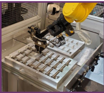
Dual Pallet Station w/ Horizontal Presentation
