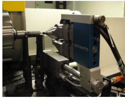
Automatic in-process sizing gage
