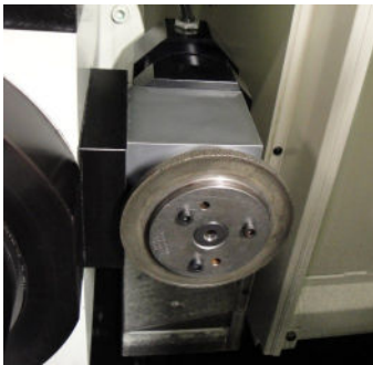
Variable speed rotary dresser
