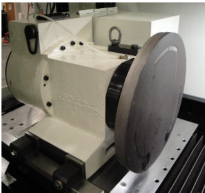
Heavy-duty workhead with custom vacuum chuck assembly
